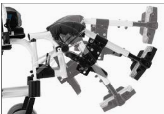
Pedane elevabili estraibili. Detachable elevating footrests.
